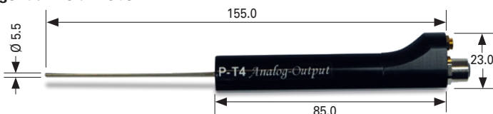
Tangential Field Probe P-T4A:
