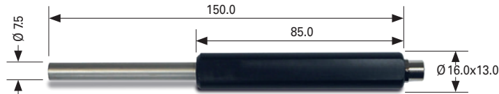
Tangential Field Probe P-T2/T4: 1.7 mm thickness
