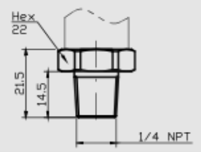
1/4 " NPT
