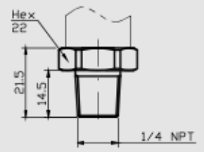
1/4 " NPT
