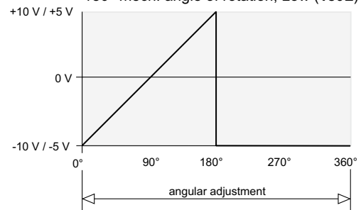
180° mech. angle of rotation, Low (180L)
