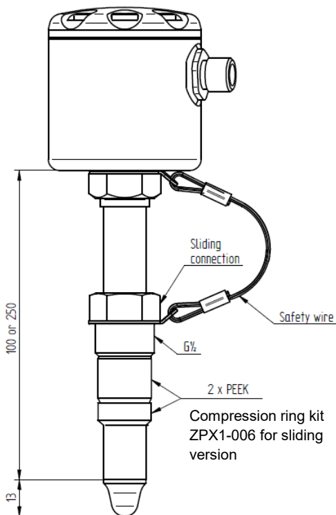
G 1/2 A hygienic sliding connection
