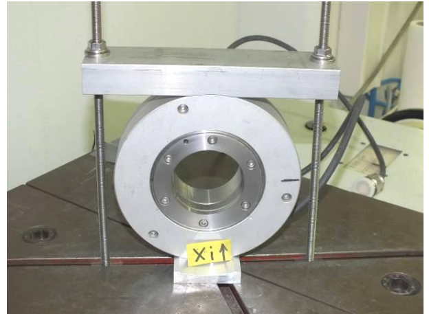
picture 8 Incremental Encoder HOGS 151 on the shock table with acceleration sensor during and shock test in X-axis, negative direction
