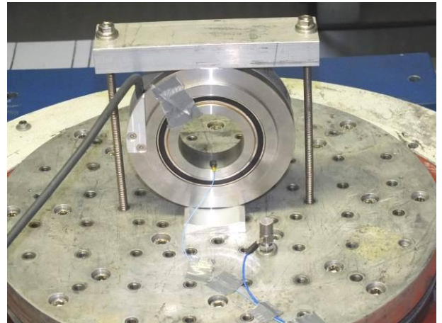
picture 2 Incremental Encoder HOGS 151 on the vibration table with acceleration sensors during vibration test in X-axis
