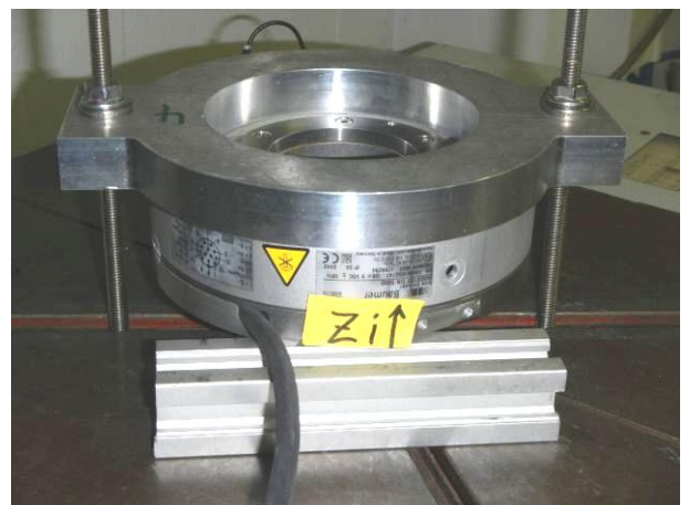
picture 12 Incremental Encoder HOGS 151 on the shock table with acceleration sensor during shock test in Z-axis, negative direction
