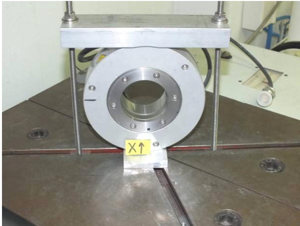
picture 7 Incremental Encoder HOGS 151 on the shock table with acceleration sensor during shock test in X-axis, positive direction
