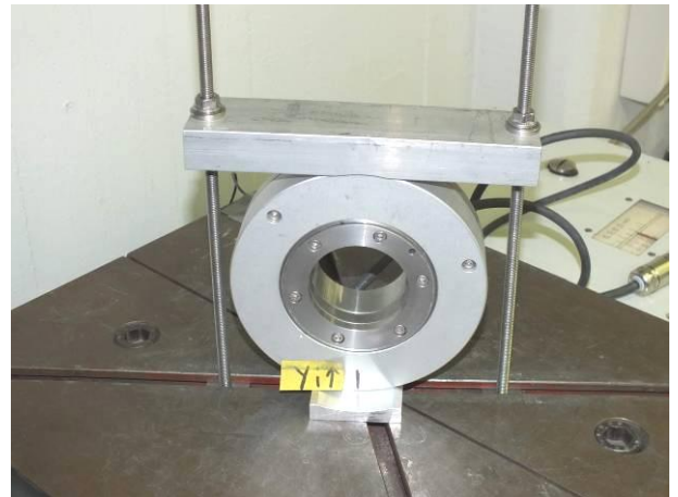
picture 10 Incremental Encoder HOGS 151 on the shock table with acceleration sensor during shock test in Y-axis, negative direction
