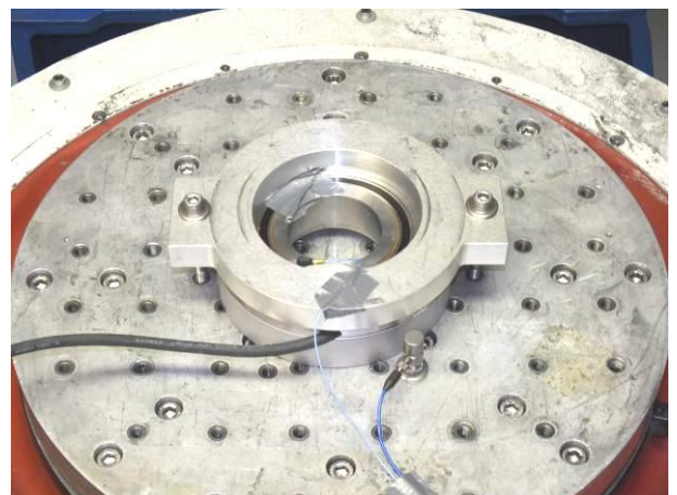
picture 6 Incremental Encoder HOGS 151 on the vibration table with acceleration sensors during vibration test in Z-axis
