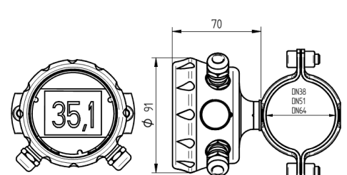
Tube mounting
