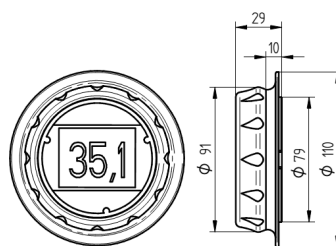
Panel mounting
