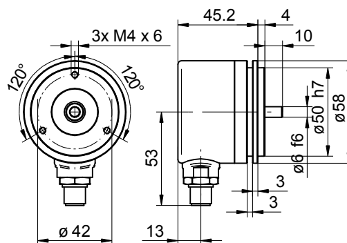
EAM580R-SY with flange connector M12
