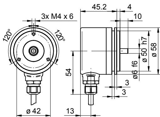
EAM580R-SY with cable
