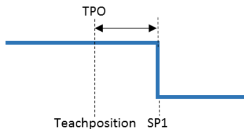
Figure 24: O200.G/O200.R: Single Point Teach, switching behavior
