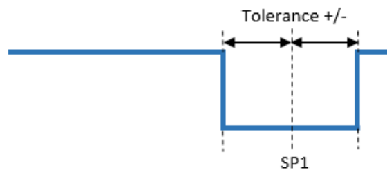
Figure 25: O200.S: Single Point Teach, switching behavior
