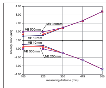
typical linearity error
