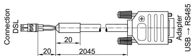
Connecting cable for DSL-RS485 interface
