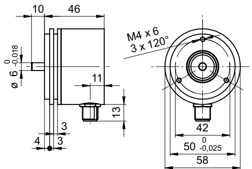
BRIV 58S, connector output M12 radial
