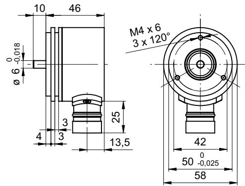
BRIV 58S, connector output M23 radial
