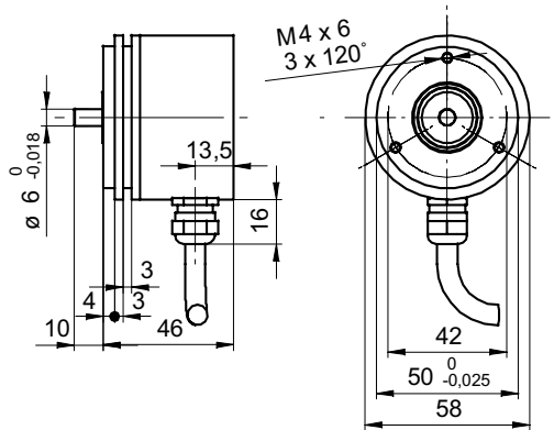
BRIV 58S, cable radial
