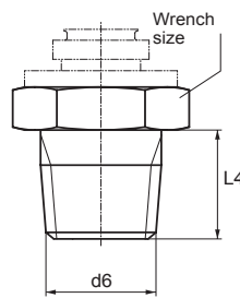
Conical screw threads
