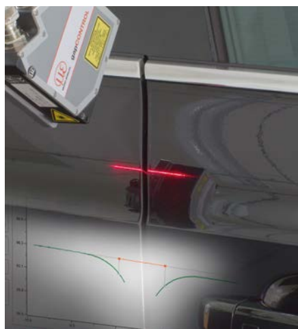
Gap and flushness measurement on bodywork parts
