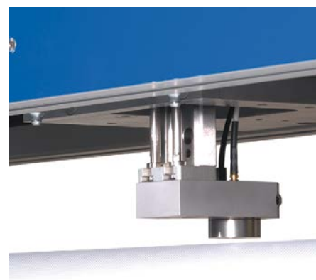
Non-contact, inline thickness measurement of plastic films
