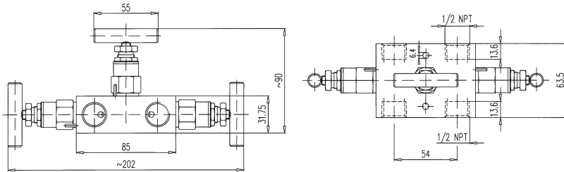
Manifold 3 ways
